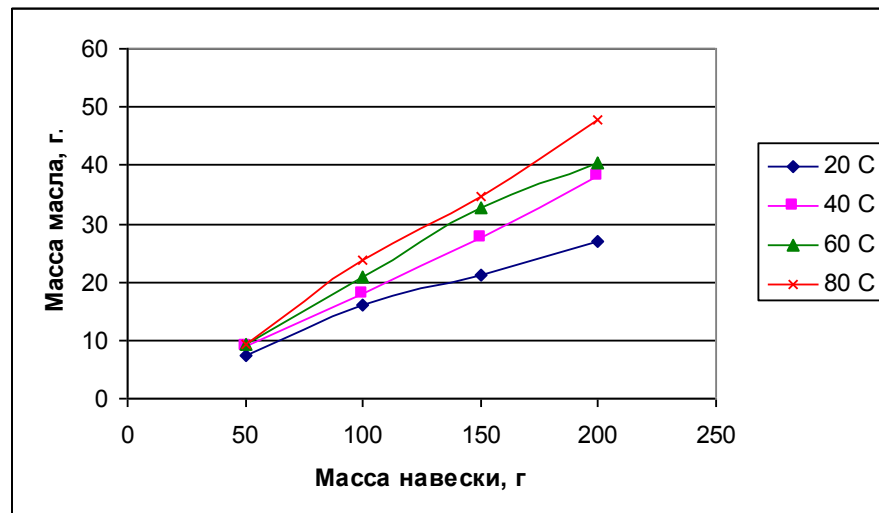
Figure 1. Influence of the seed load on the mass of the collected oil
